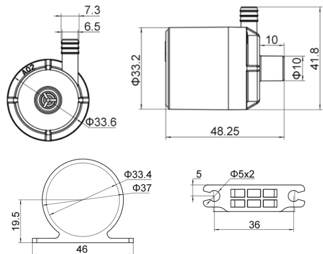
Dimension (mm)
