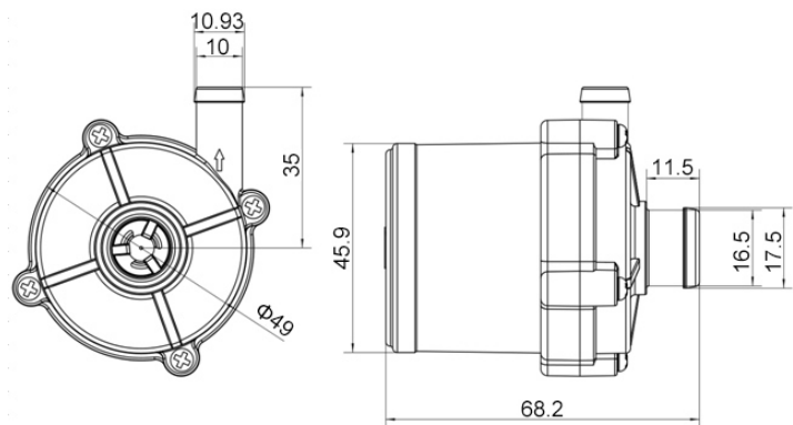
Dimension (mm)
