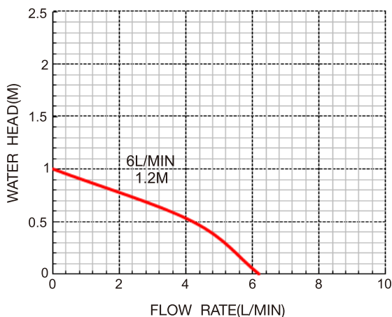
TL-B09 Performance
