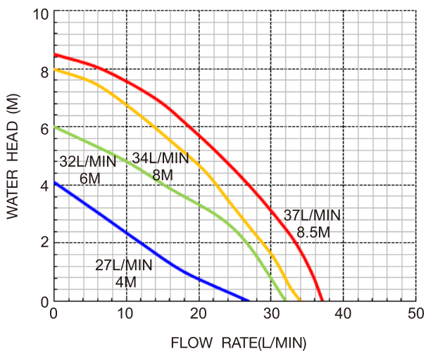
TL-C02 Performance
