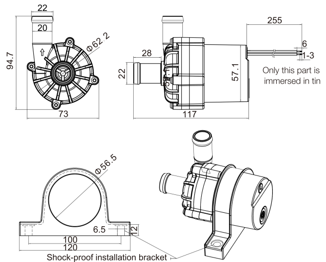
Dimension (mm)
