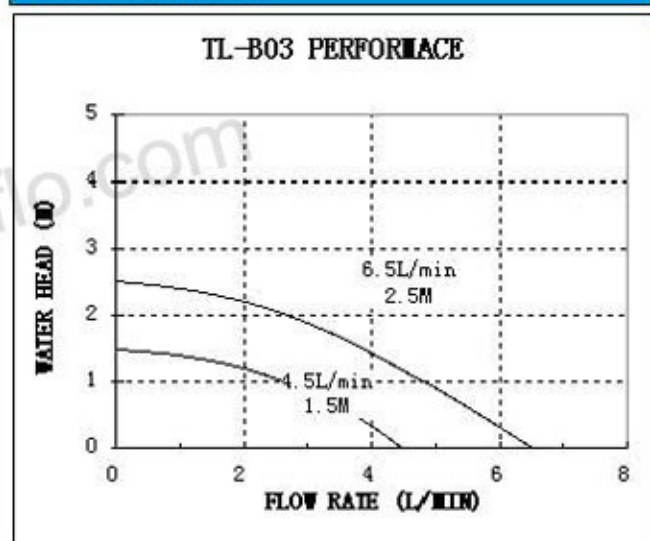
TL-B03 curve
