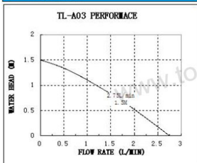
TL-A03 curve
